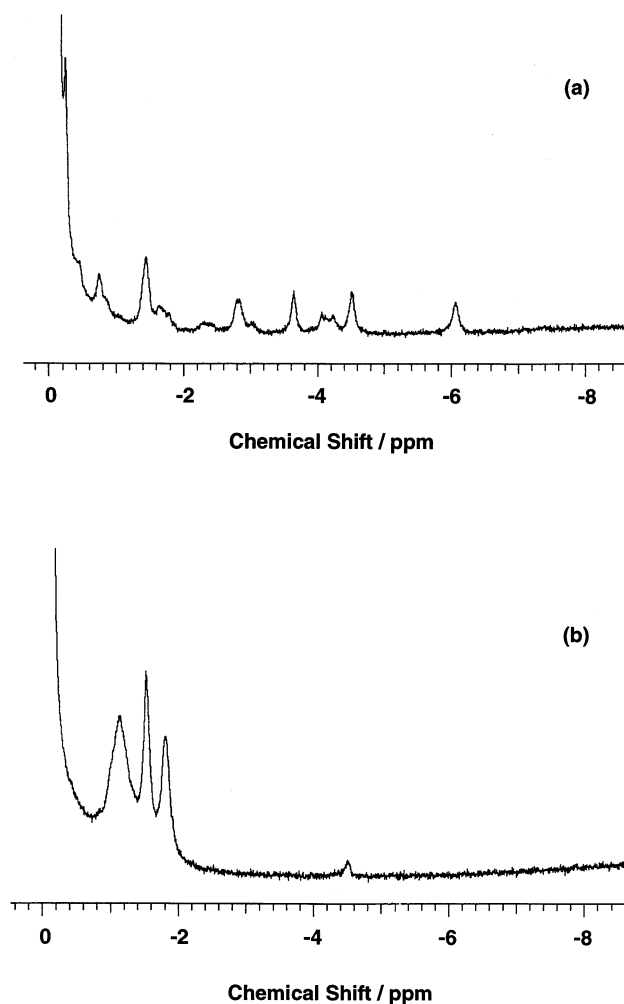
Fig. 6. ^1\text{H} -NMR spectra of (a) ferrous CooA and (b) CO-bound CooA. CooA (700 \mu\text{M} of the dimer) was dissolved in a 50 mM \text{KH}_2\text{PO}_4 –NaOH buffer (pH 7.6).
